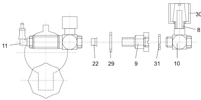
Detail SEV
