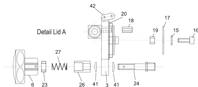
Detail Locking
